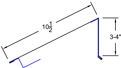
High Eave with clip and Z closure
